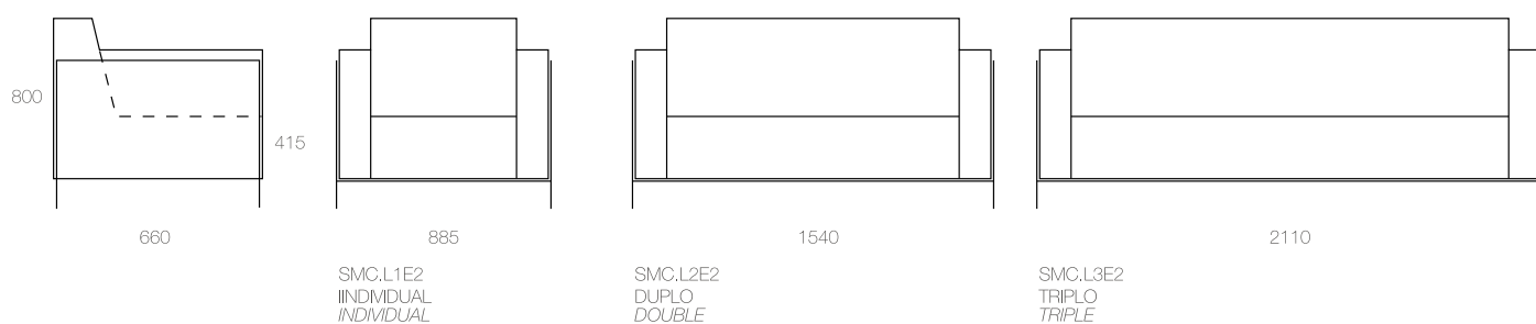
PUF VISTA LATERAL LATERAL VIEW
